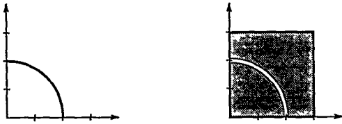
Figure 5: The non-semi-linear semi-algebraic sets of Example 4.2.
