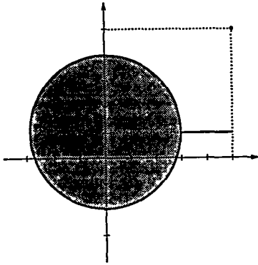
Figure 2: The semi-algebraic set of Example 3.1.
