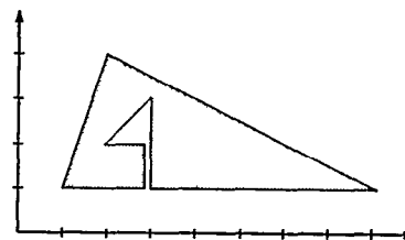
Figure 4: The semi-linear set of Example 3.7.
