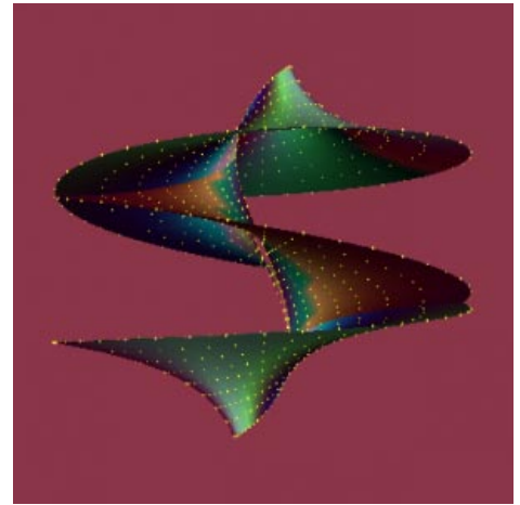
Figure 8: z_1 (z_2)^2 = 1
