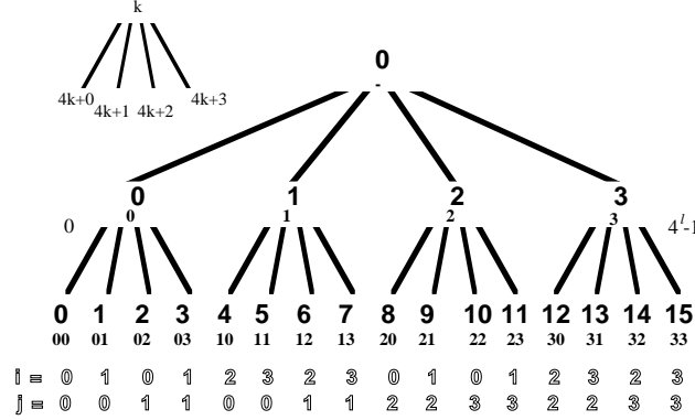
Figure 2: Morton indexing of the order-4 quadtree [35].
