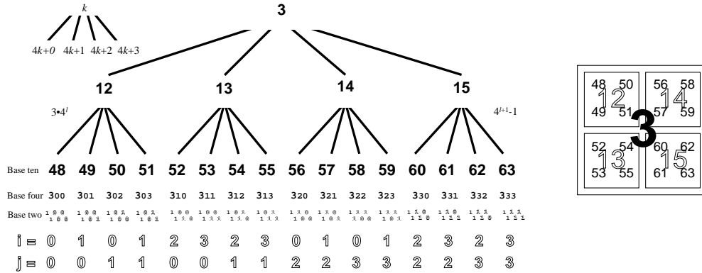
Figure 4: Ahnentafel indexing of the order-4 quadtree.
