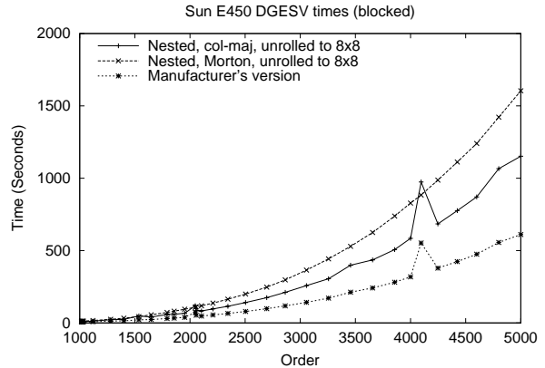
Figure 6: Uniprocessor running times for dgesv compiled to Morton-order matrices.
