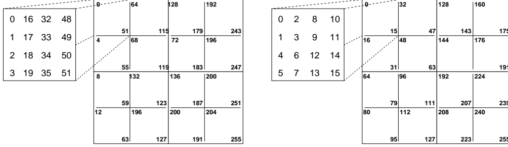
Figure 1: Column-major indexing of a 16 \times 16 matrix, and analogous Morton indexing.
