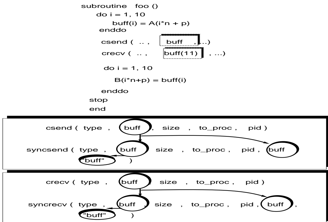
Figure 2: Transformation of communication calls during instrumentation. Top: the original program; Bottom: the communication call is replaced with a call to a monitor library routine with two additional fields.
