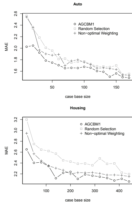
Figure 3: MAE of AGCBM1 and two variants in two sample domains
