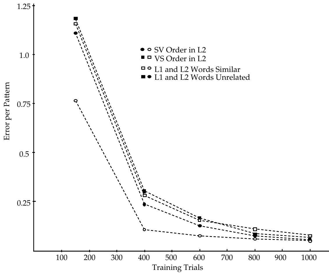
Figure 5: Sum-of-Square Errors for L2 Patterns
