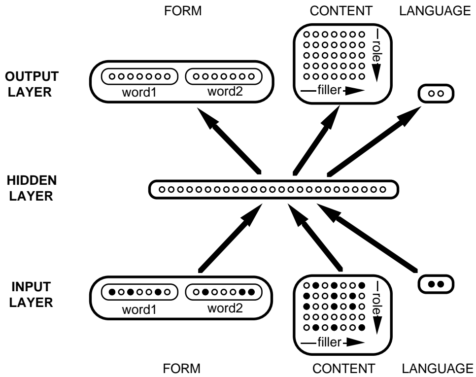
Figure 1: Architecture of Network Used in Simulations
