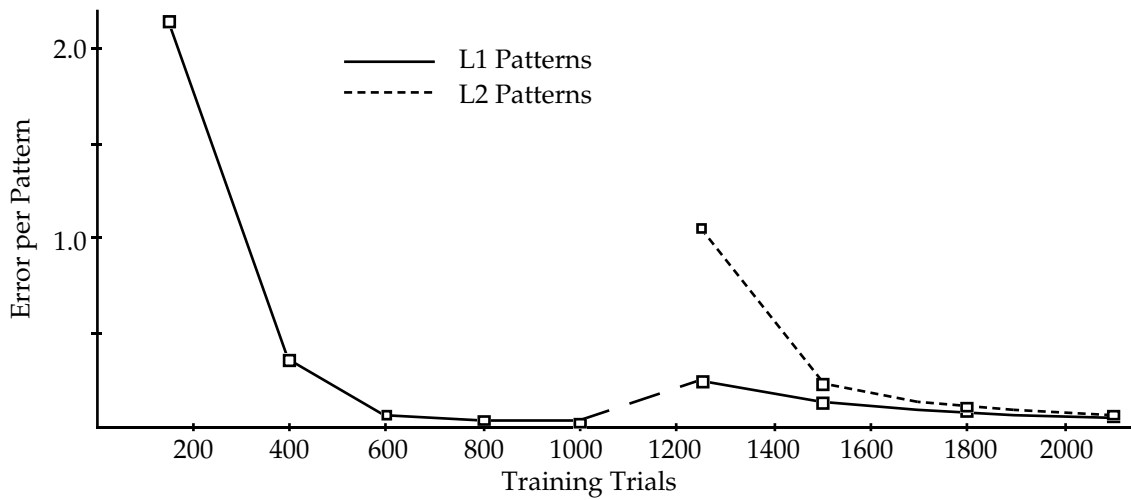
Figure 2: Sum-of-Square Errors for L1 and L2 Patterns
