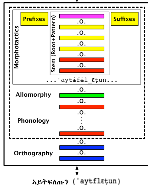
Figure 3: Architecture of the system. Rectangles represent FSTs, “.o.” composition.
